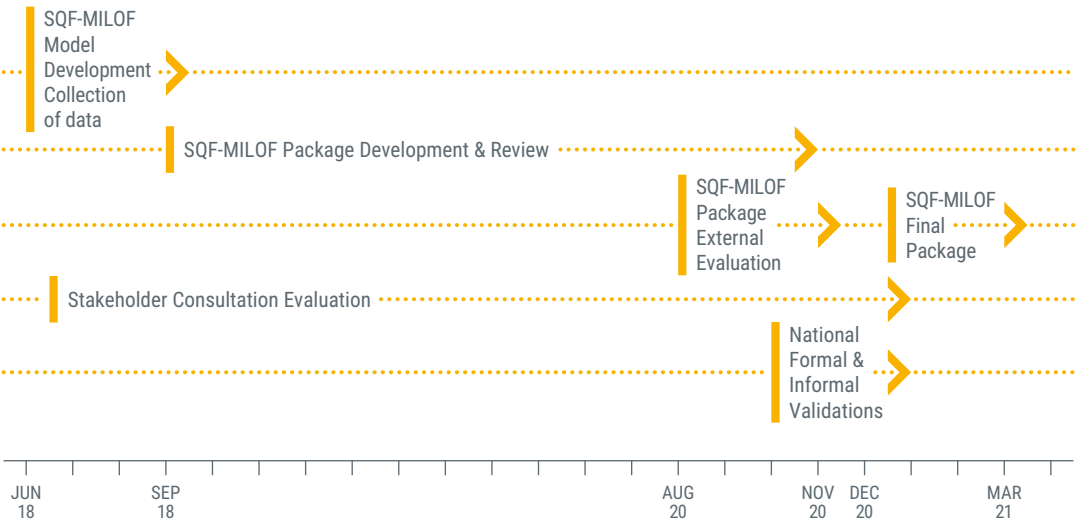
FIG.2 - SQF-MILOF TIMELINE
